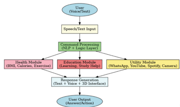
Figure 1: AI Assistant System Methodology
